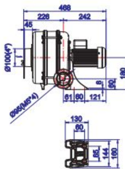
HTB75-053 3-stage
