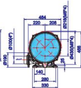
HTB100-505 5-stage
