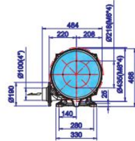
HTB100-203 3-stage
