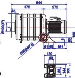
HTB75-105 5-stage
