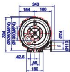
HTB75-105 5-stage
