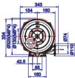
HTB75-053 3-stage
