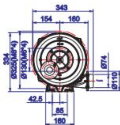
HTB75-104 4-stage
