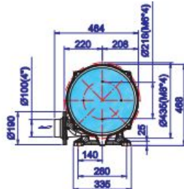
HTB100-304 4-stage
