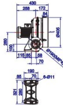
HTB100-102 2-stage
