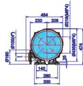
HTB100-102 2-stage
