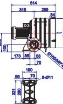
HTB100-304 4-stage
