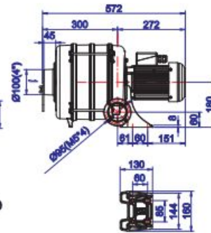
HTB75-104 4-stage
