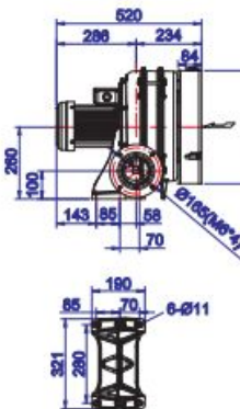
HTB100-203 3-stage
