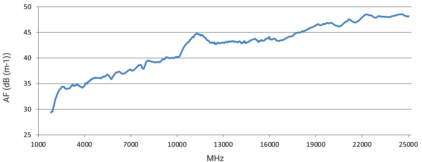
Antenna Factor Diagram HyperLOG ® PRO 18250
