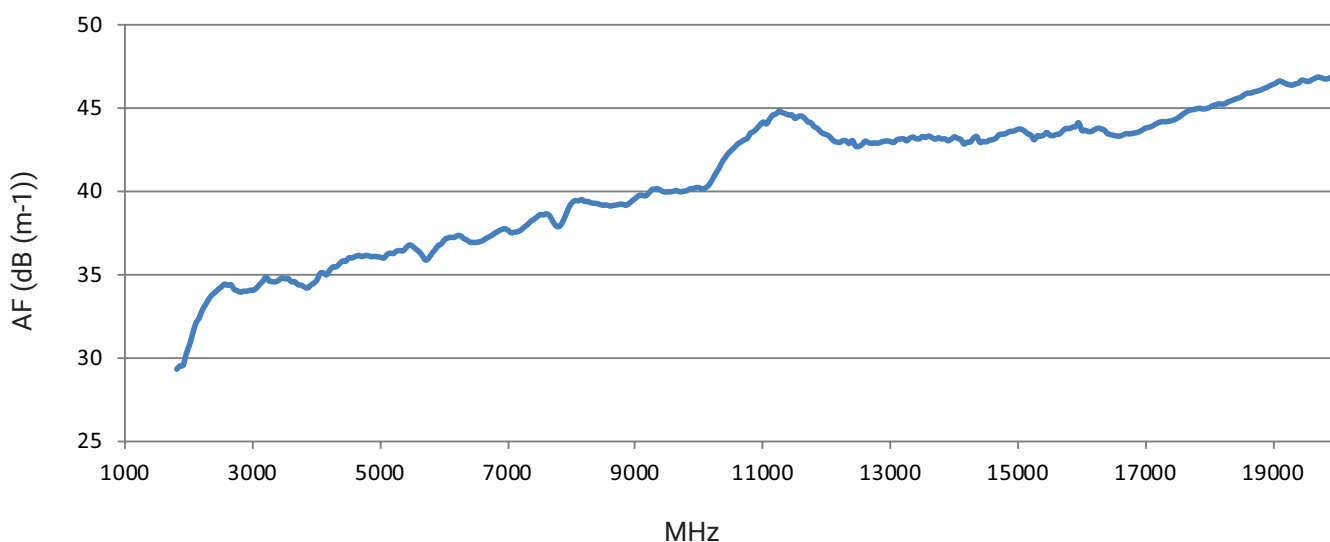
Antenna Factor Diagram HyperLOG® PRO 18200
